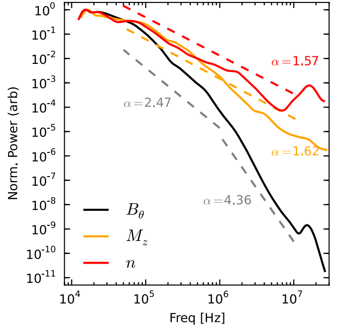
Figure 4. Wavelet spectrum of B -field, density, and Mach number fluctuations for the equilibrium epoch, 40–60 \mu s.
